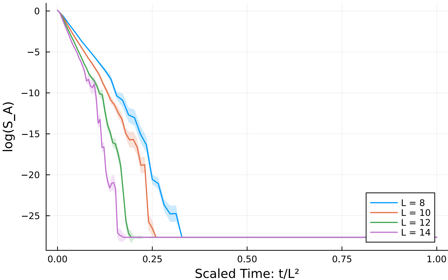
Scaled Log Entropy Evolution ( p = 0.750000 )
